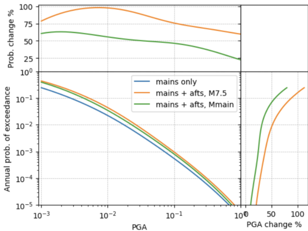
Figure 6 - Hazard curves for the METIS test site, considering three scenarios: The mainshock-only hazard curve is shown in blue. The scenario with the aftershock M_{max} = 7.5 for all sequences is shown in orange. The scenario with the aftershock M_{max} = M_{main} is shown in green.
